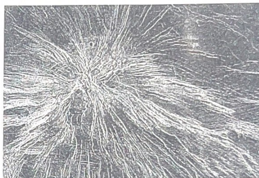
Novae are dome-shaped landforms on Venus. They are easy to see from above because they have cracks reaching out from their centers in all directions. The word novae is the plural form of the word nova .
